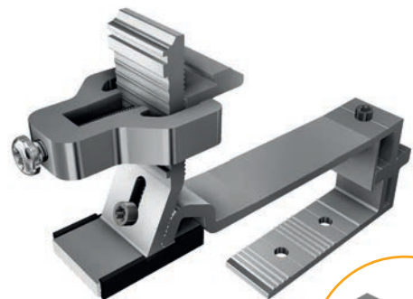
SL Alu Multi Hook Item no. 11100-05
