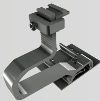
Roof hooks SL: From 35- 65 mm
