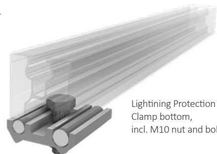
Lightning Protection Clamp top, very low height, suitable for 30 mm module frames
