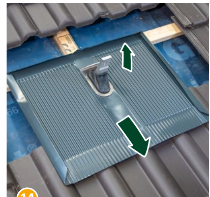
14 Align the Alpha-Plate and ensure that there are no unintentional indentations in the top and center area, which could lead to the formation of water pockets. Leave the rear sheet metal edging slightly bent forward.
