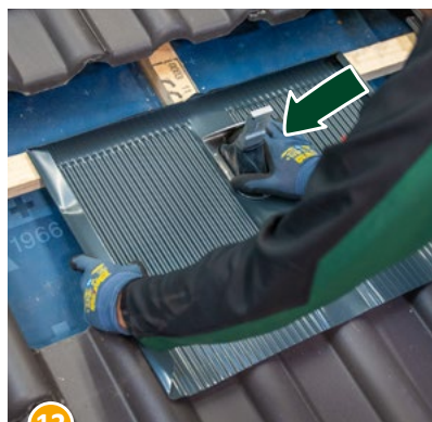
13 Place the opening in the support plate on the upper horizontal batten and put the Alpha-Plate with its riveted sealing sleeve over the console.
