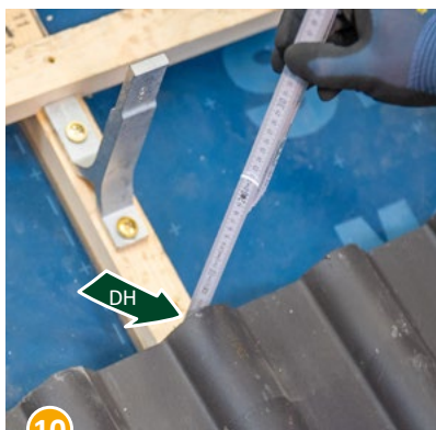
10 Determine the height of the roof tile (DH), that needs to be compensated.
